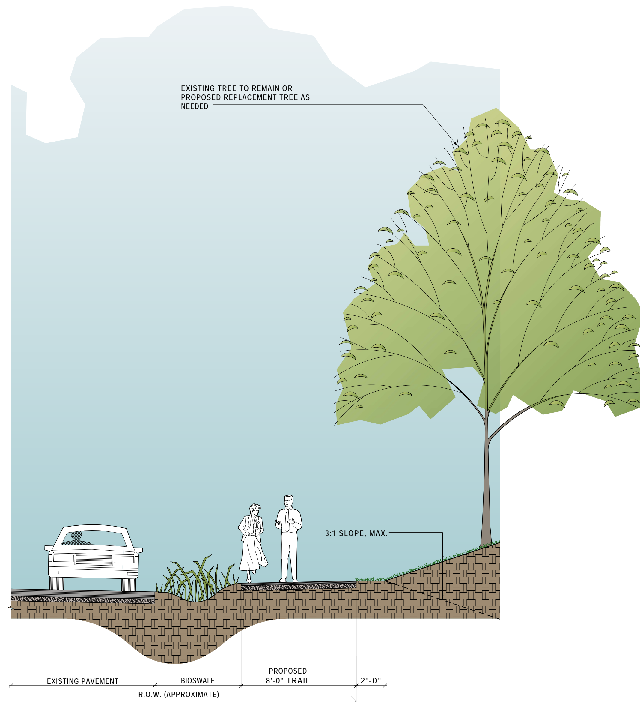
5 TYPICAL NEIGHBORHOOD CONNECTOR WITH BIOSWALE SECTION SCALE: 1/4"=1'-0" (ROAD SIGNED AND MARKED FOR BIKE BOULEVARD) @ FORD PL. @ McCORMICK ST.
