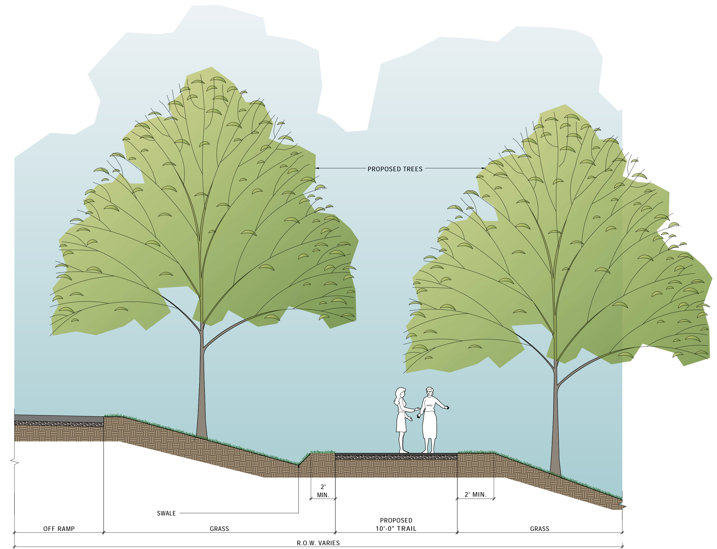
4 TRAIL ALONG OFF RAMP SCALE: 1/4"=1'-0"
