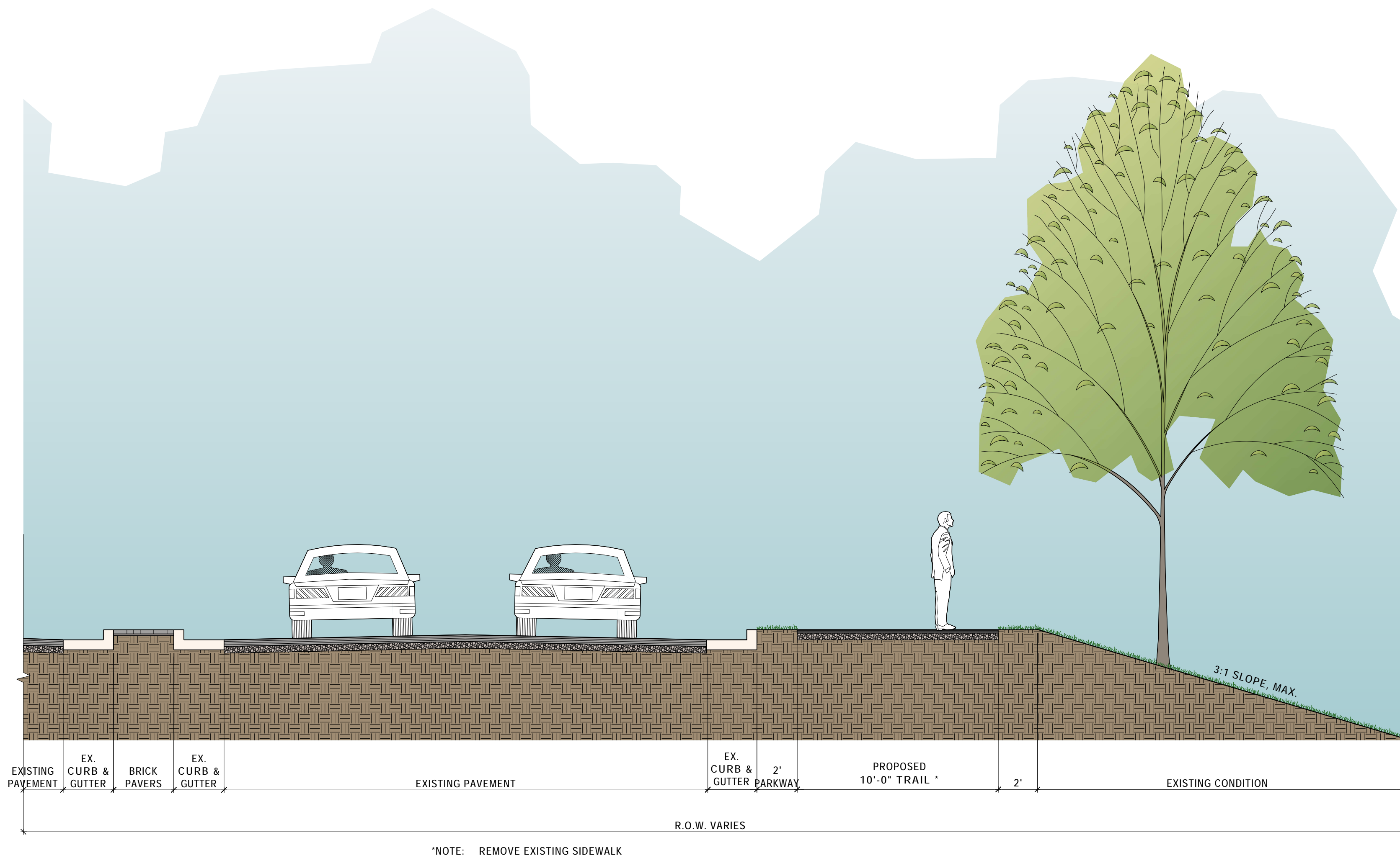
14 TRAIL ALONG MLK JR. AVENUE @ FILL SLOPE SCALE: 1/4"=1'-0"
