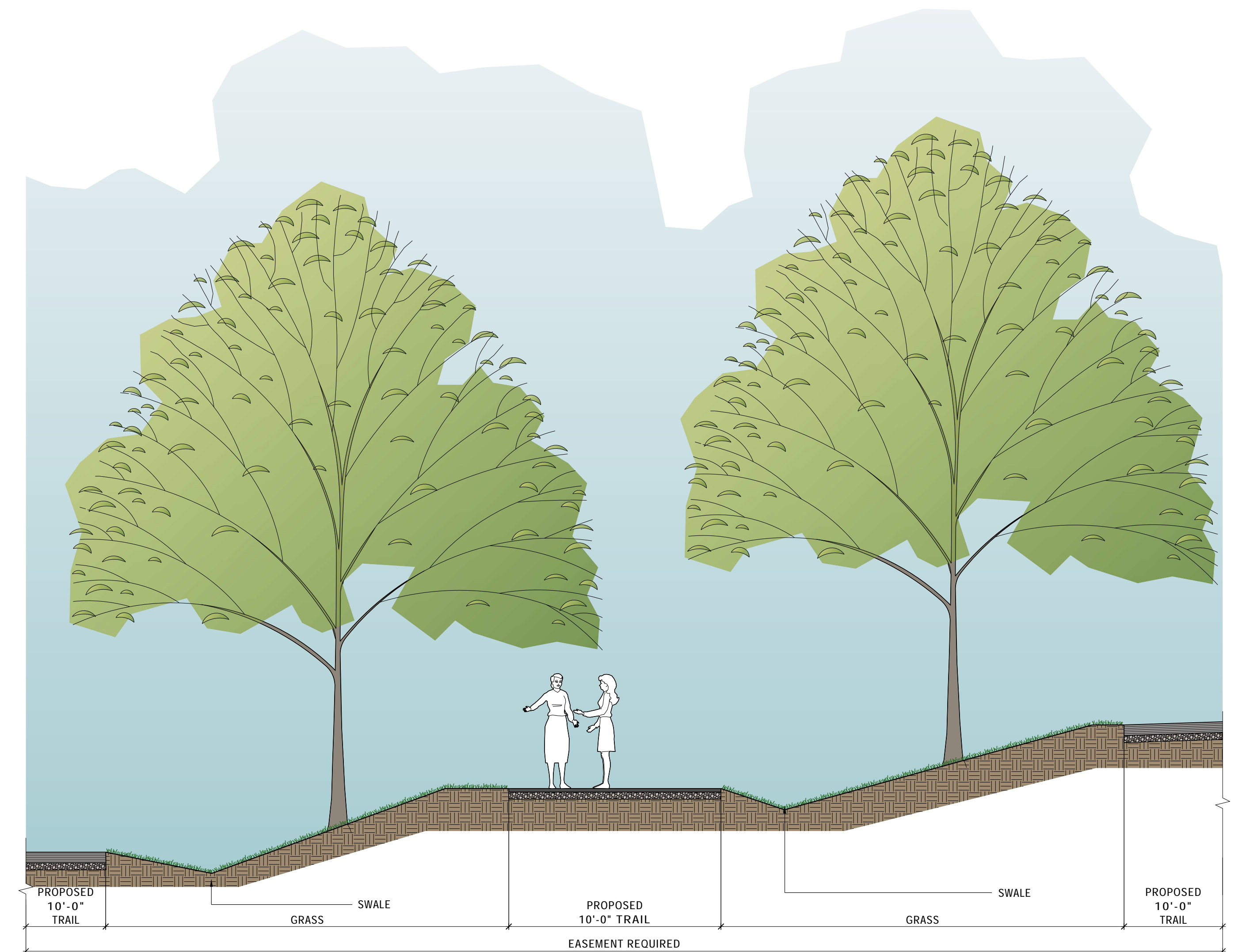
13 TYPICAL TRAIL ON SLOPE SCALE: 1/4"=1'-0"
