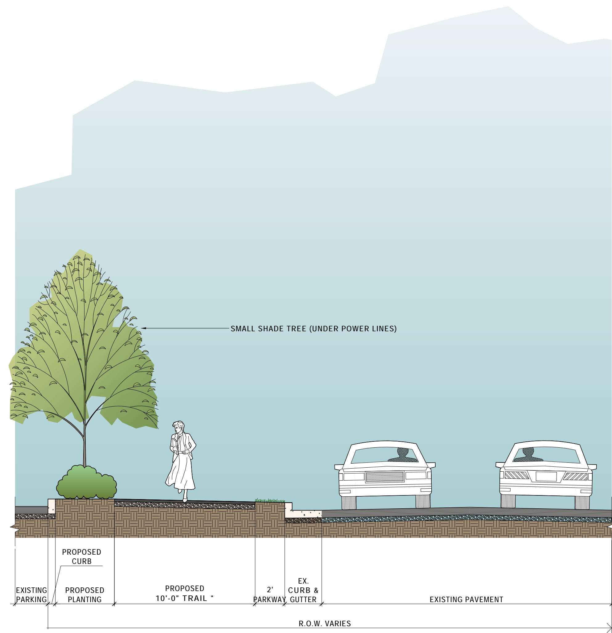
4 TRAIL SECTION ALONG BROADWAY @ PARKING LOT / DRIVEWAY SCALE: 1/4"=1'-0"
