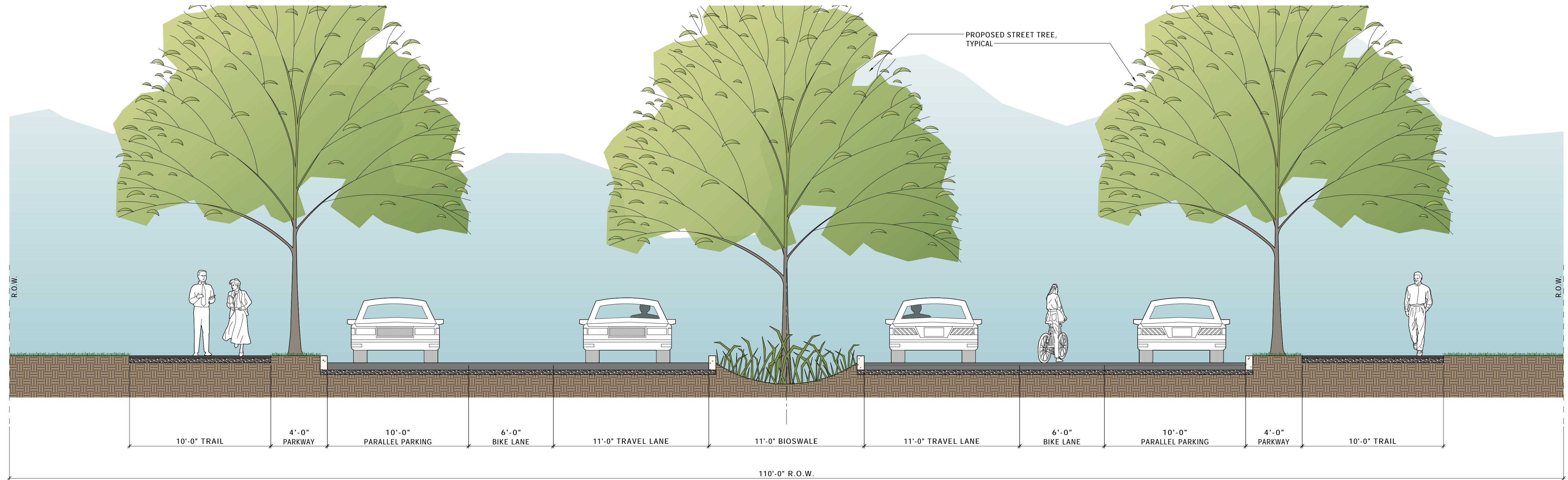
5 WALKER BOULEVARD SECTION SCALE: 1/4"=1'-0"
