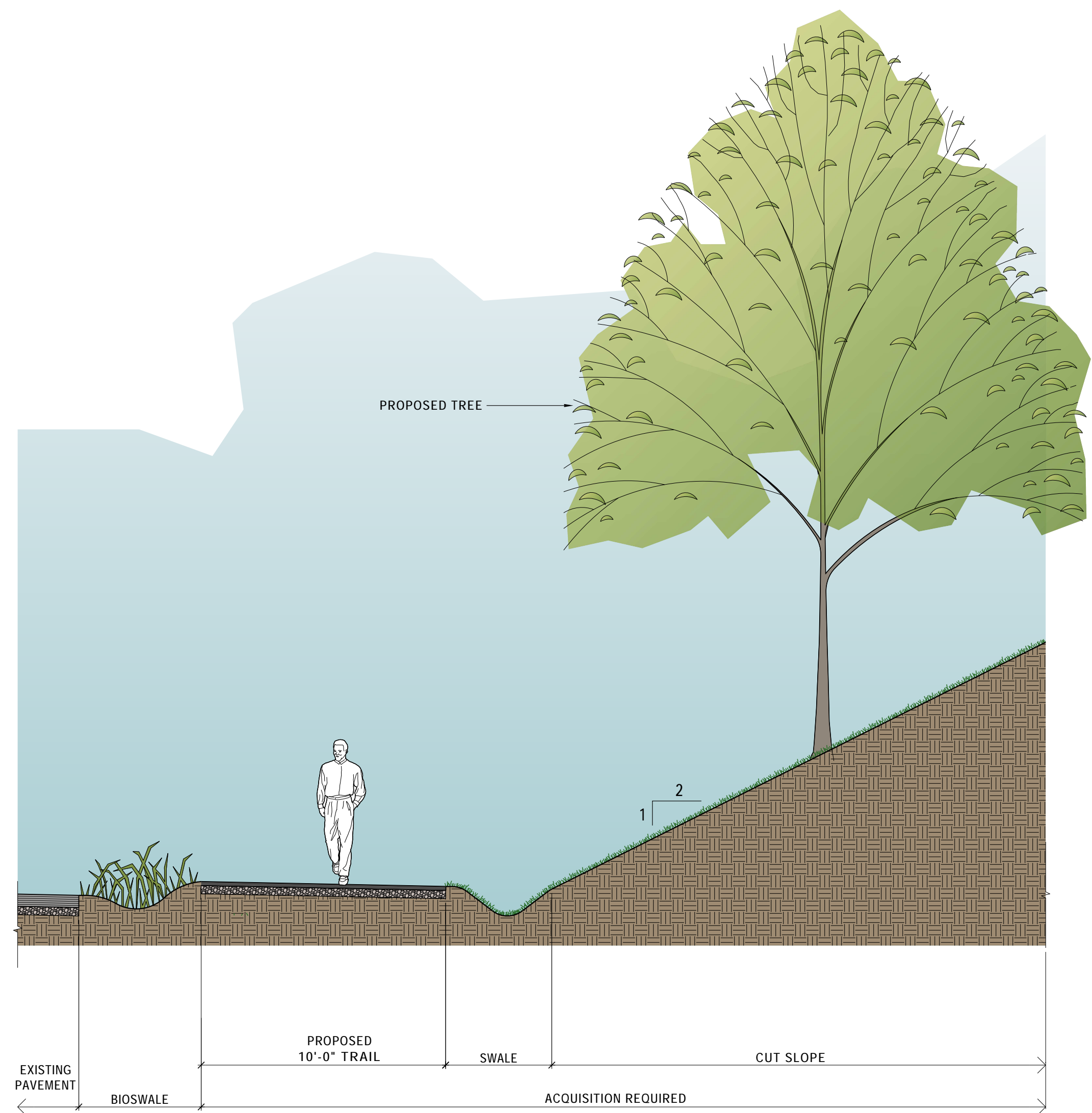
10 TRAIL SECTION @ CUT SLOPE SCALE: 1/4"=1'-0"
