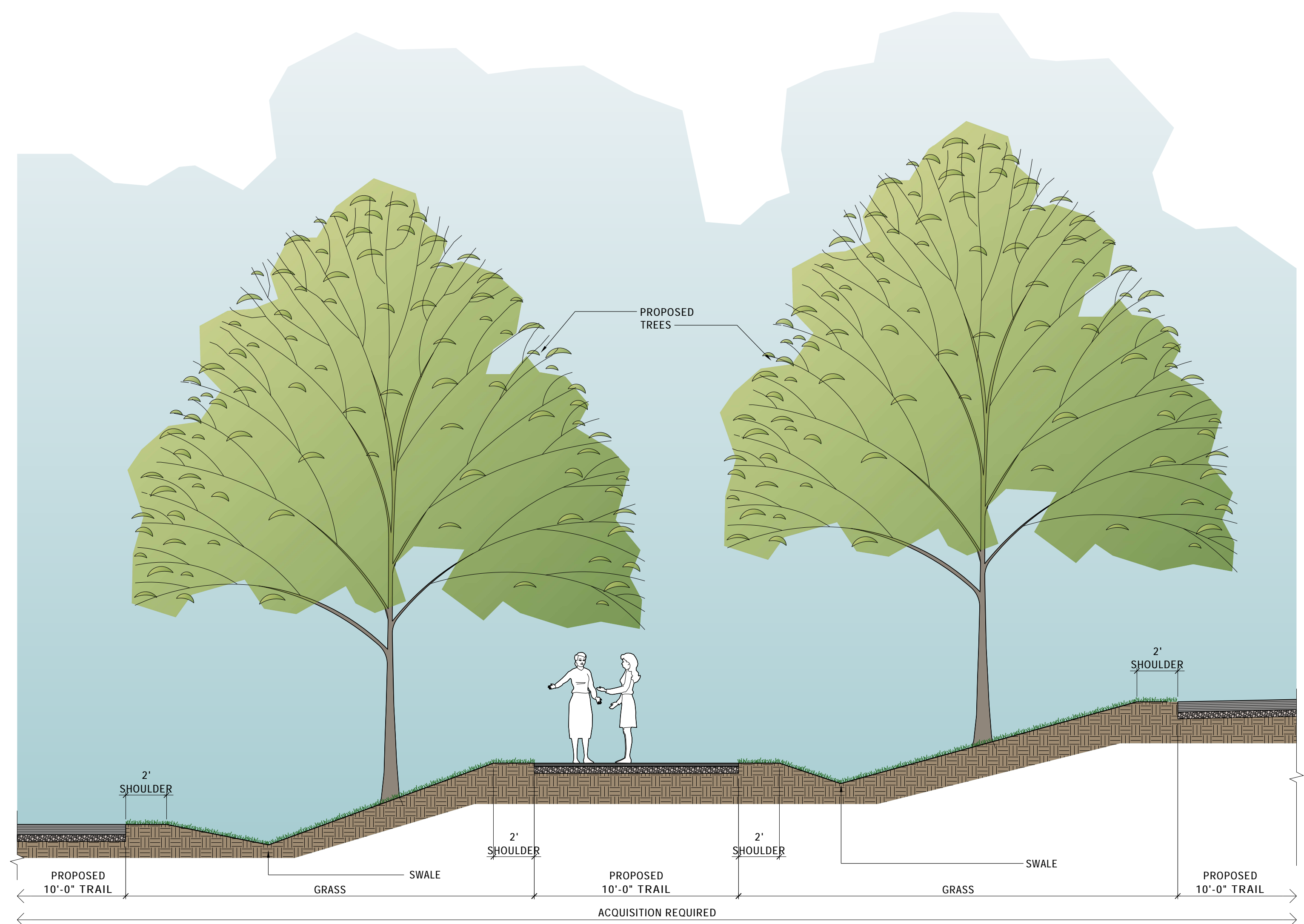
9 TYPICAL TRAIL ON SLOPE SCALE: 1/4"=1'-0"
