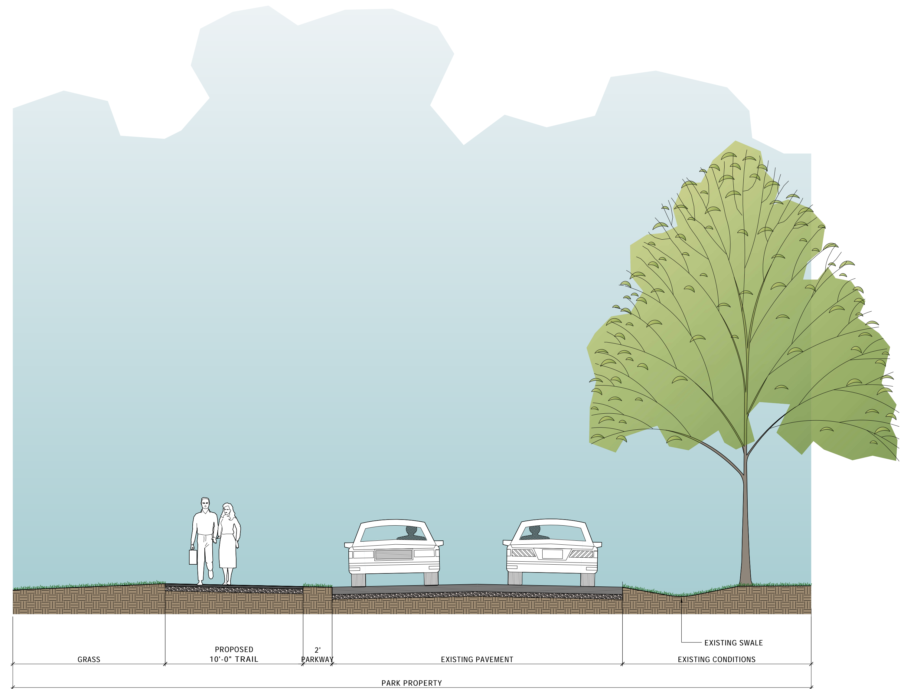
1 TYPICAL TRAIL SECTION @ DRIVEWAY SCALE: 1/4"=1'-0"
