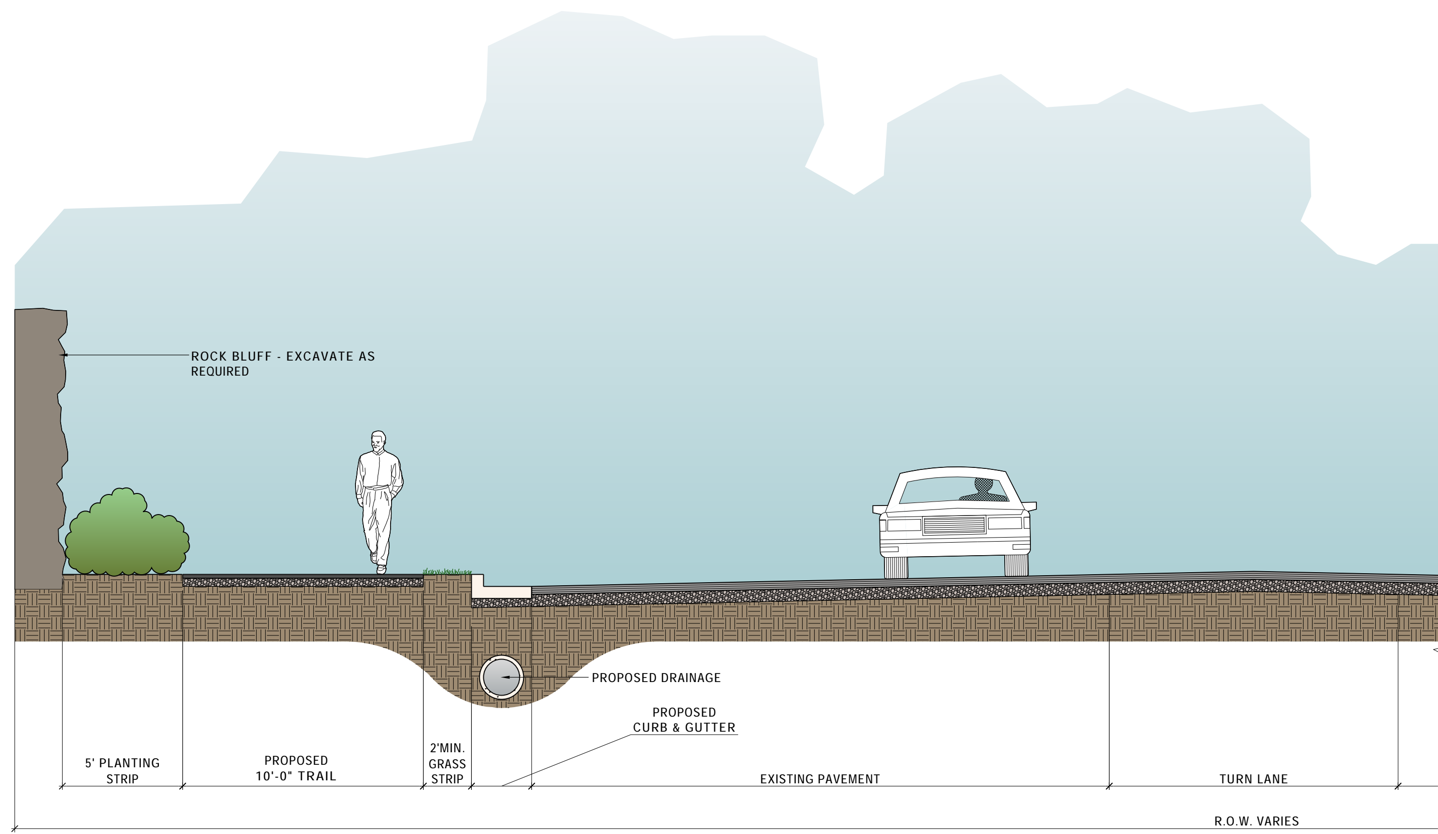
18 TRAIL ALONG NORTHSHORE DRIVE @ ROCK BLUFF SCALE: 1/4"=1'-0"
