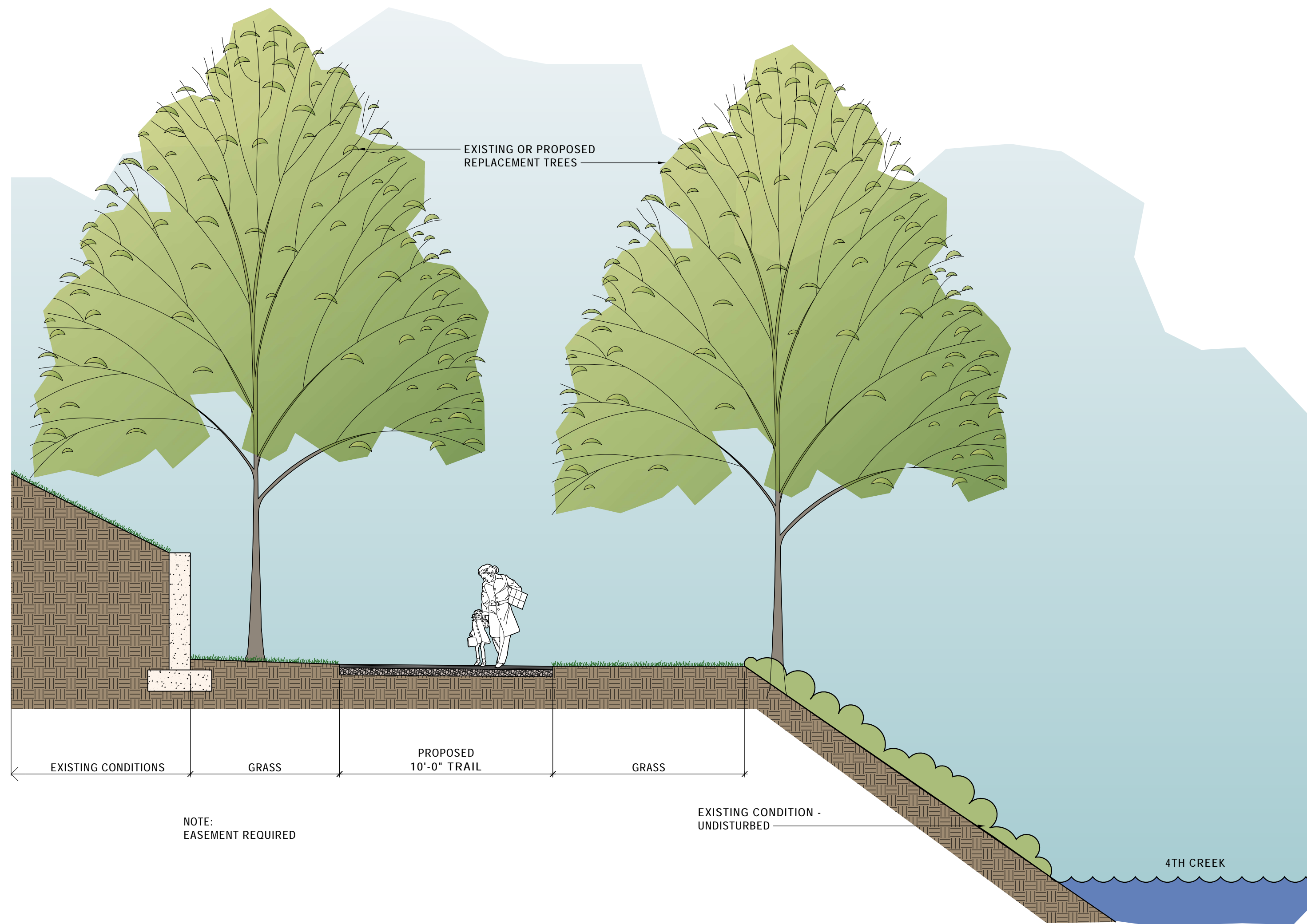
16 TYPICAL TRAIL ALONG 4TH CREEK & TRIBUTARY SCALE: 1/4"=1'-0"
