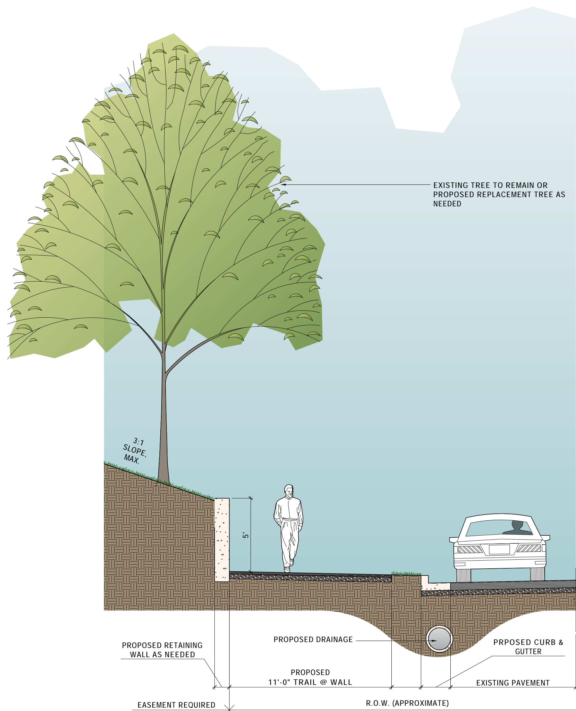
14 TYPICAL SIDEPATH SECTION @ RETAINING WALL SCALE: 1/4"=1'-0" (11' W/ NO PARKING OR PUSH BACK RETAINING WALL)
