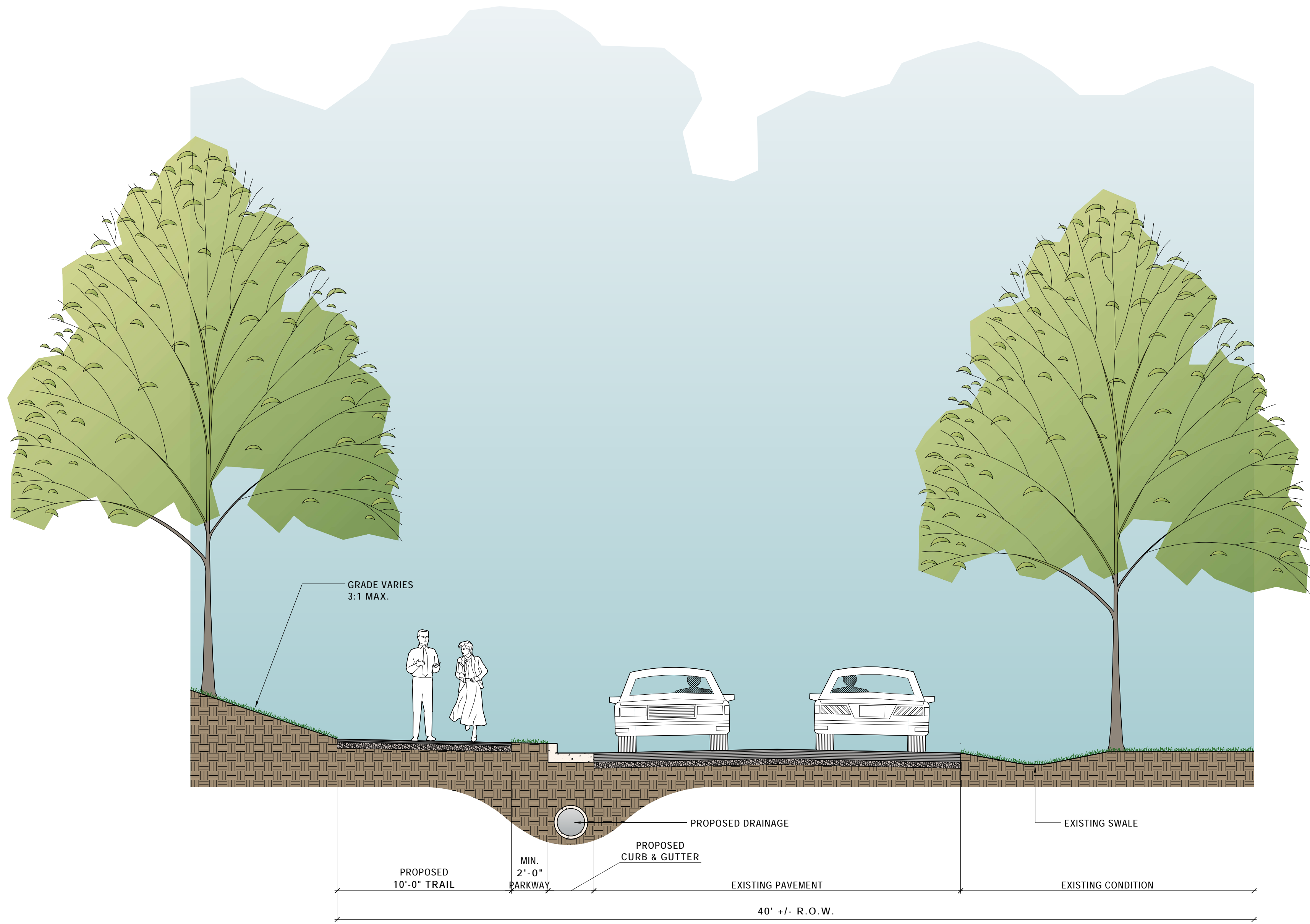
13 TYPICAL TRAIL SECTION WITH CURB, GUTTER & DRAINAGE SCALE: 1/4"=1'-0"
