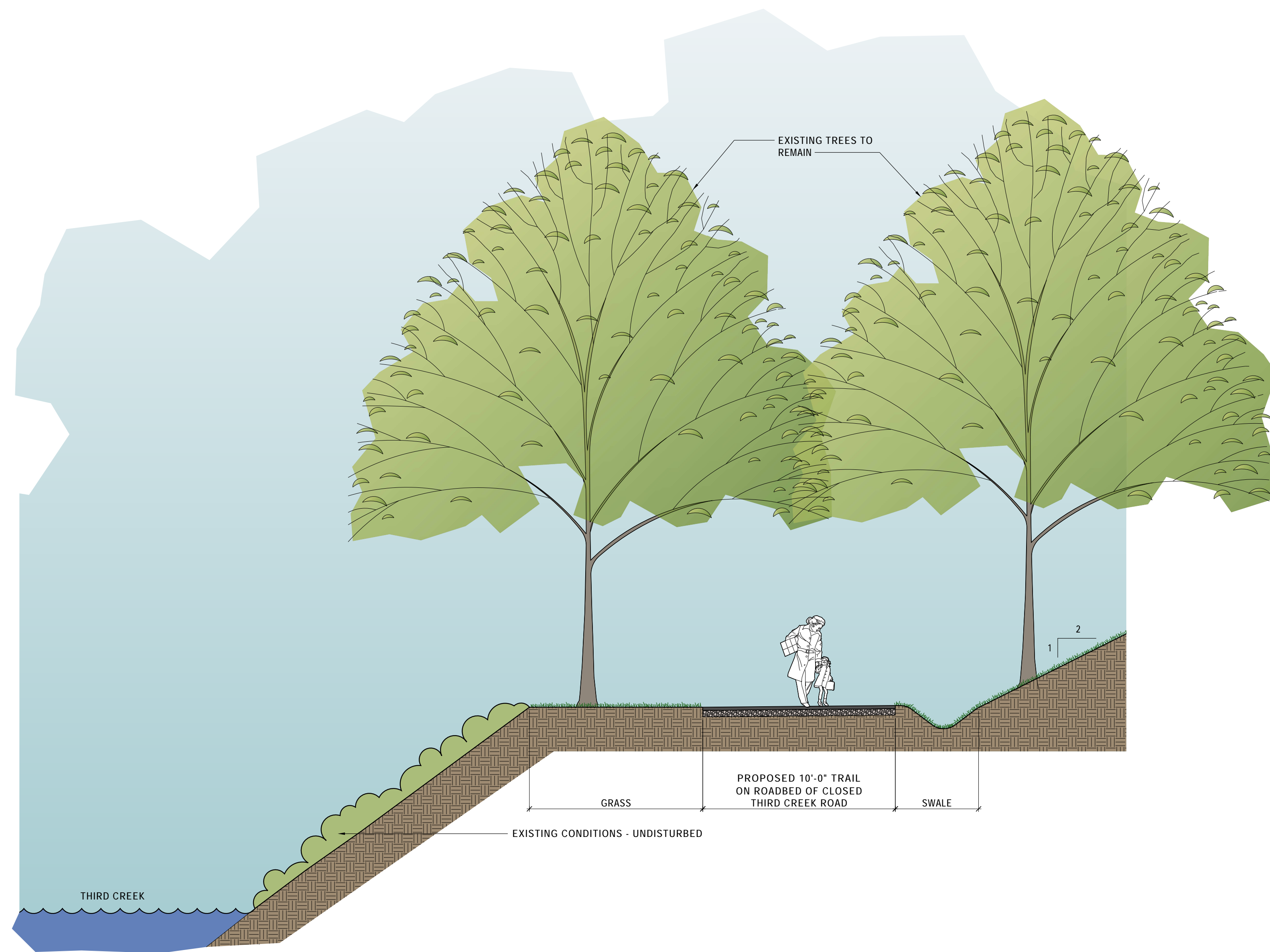
12 TRAIL ALONG THIRD CREEK SCALE: 1/4"=1'-0"
