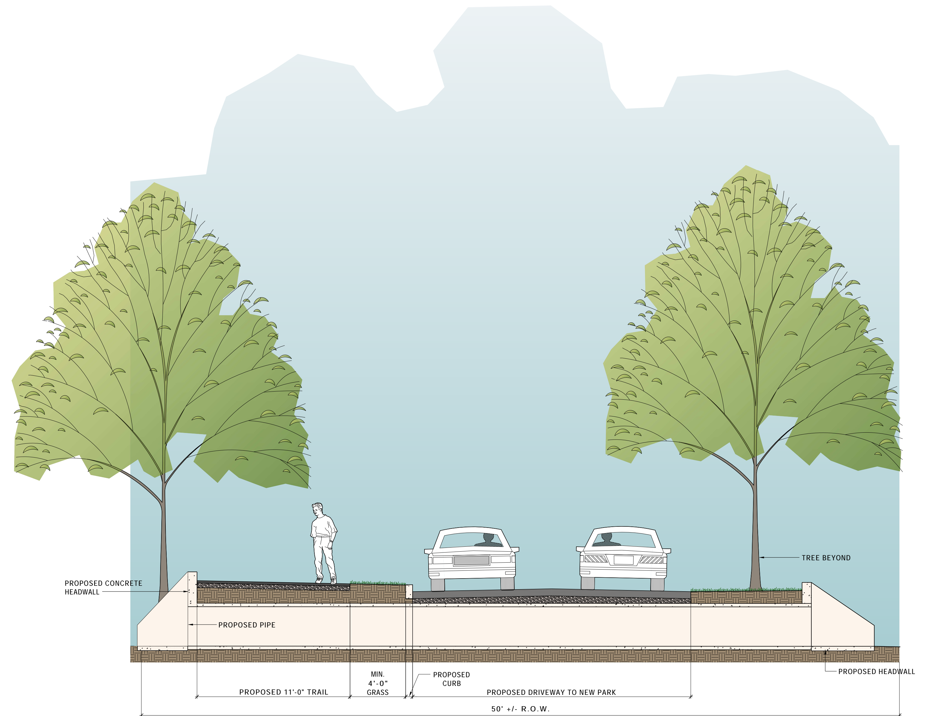
5 TRAIL SECTION @ PARK ACCESS DRIVEWAY SCALE: 1/4"=1'-0"
