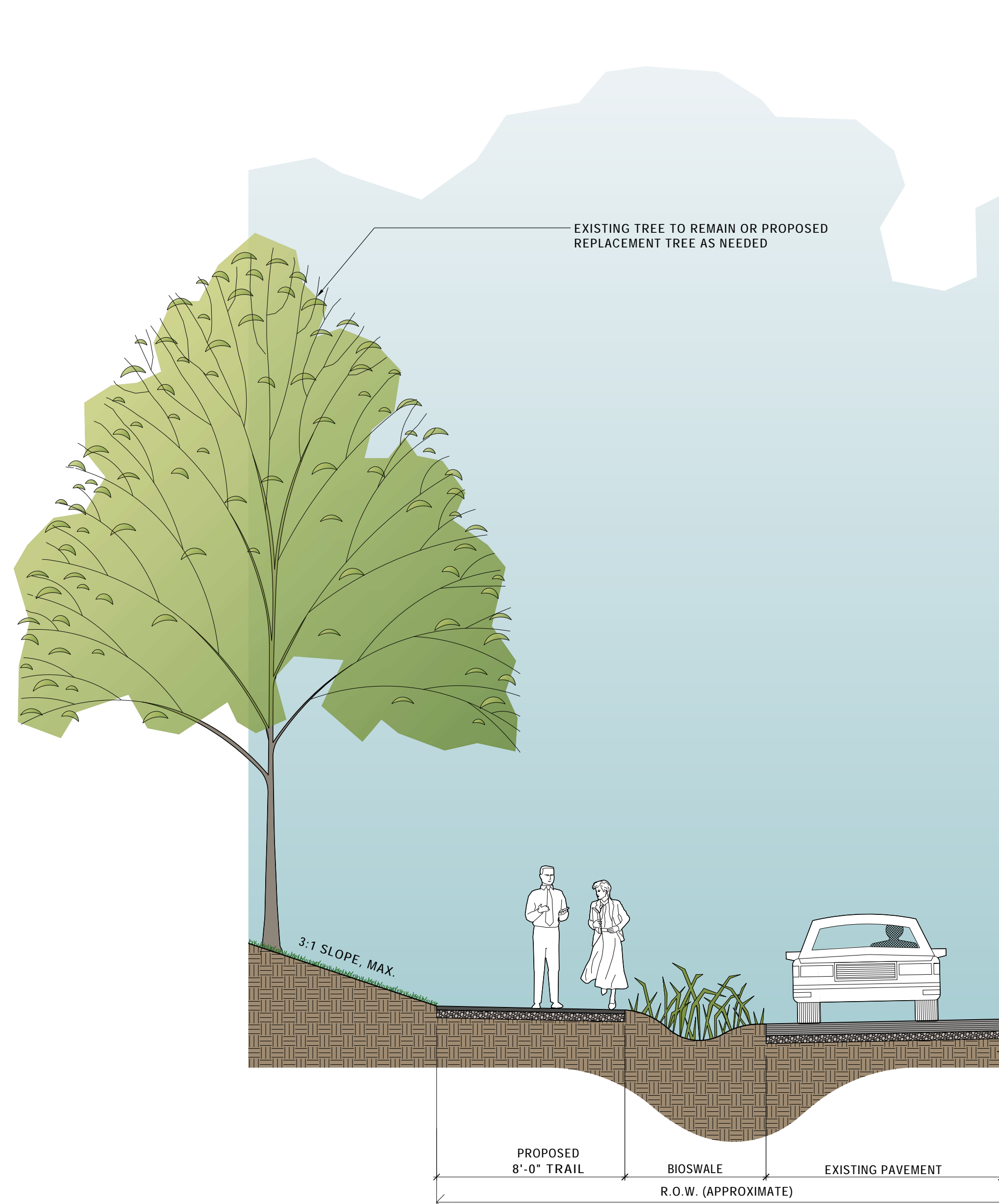
6 TYPICAL NEIGHBORHOOD CONNECTOR WITH BIOSWALE SECTION SCALE: 1/4"=1'-0" (ROAD SIGNED AND MARKED FOR BIKE BOULEVARD) @ WEST HILLS ROAD (OPPOSITE HAND) @ HAMPSHIRE DRIVE
