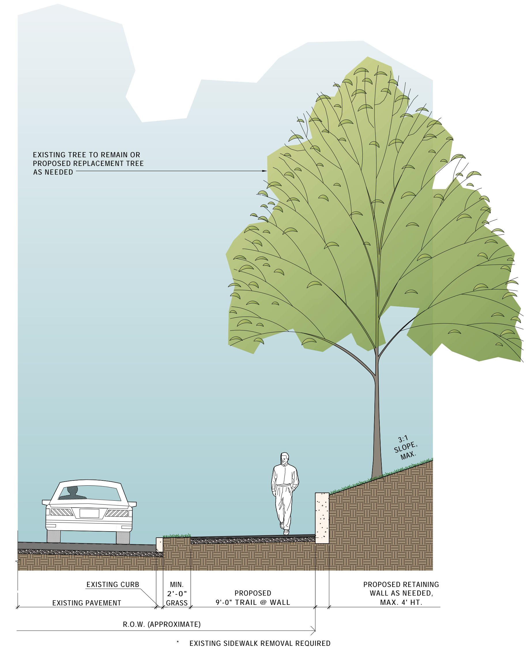
3 TYPICAL NEIGHBORHOOD CONNECTOR SECTION @ RETAINING WALL SCALE: 1/4"=1'-0" (ROAD SIGNED AND MARKED FOR BIKE BOULEVARD) @ WESTRIDGE DRIVE
