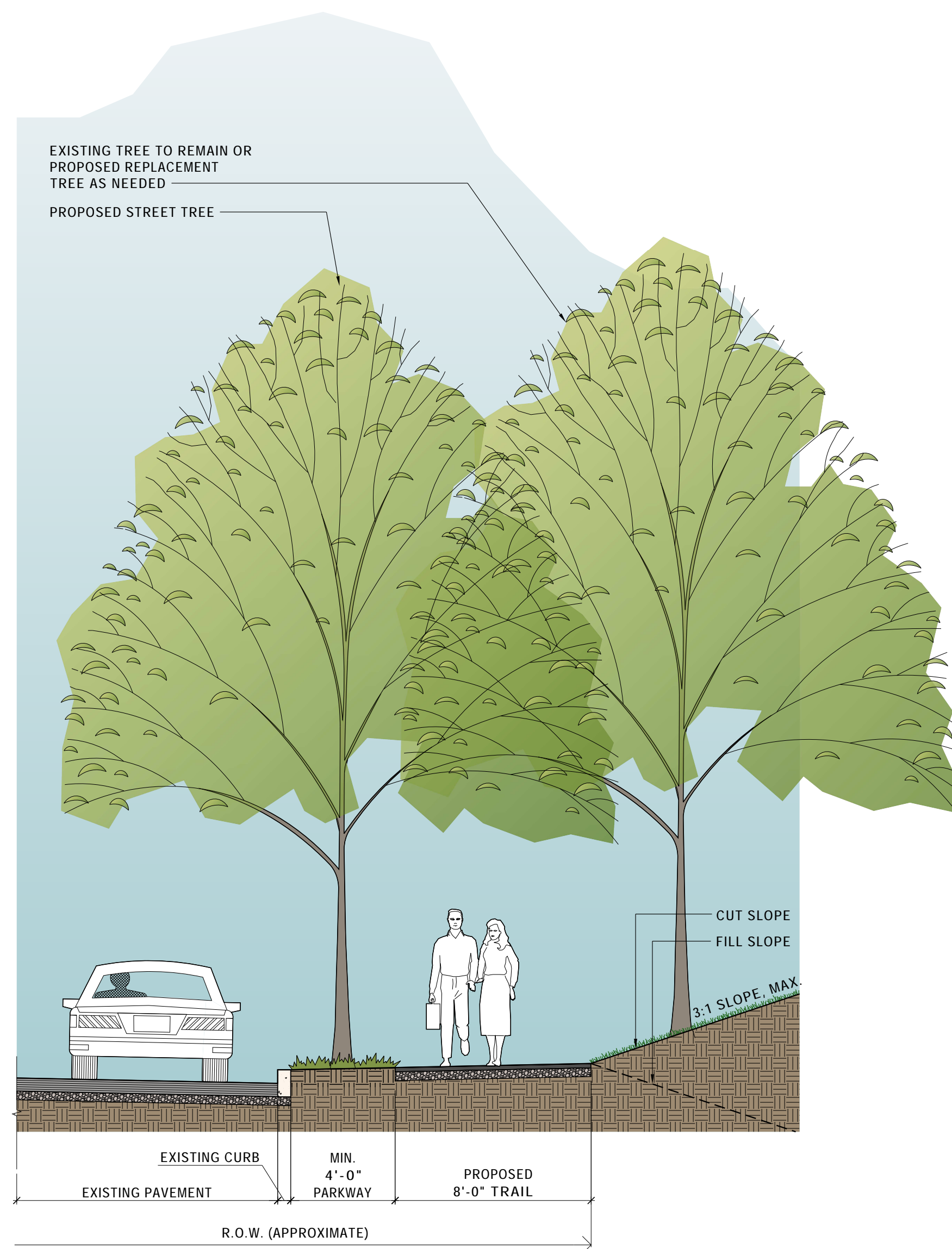
2 TYPICAL NEIGHBORHOOD CONNECTOR WITH PARKWAY SECTION SCALE: 1/4"=1'-0" (ROAD SIGNED AND MARKED FOR BIKE BOULEVARD) @ WESTRIDGE DRIVE @ HAMPSHIRE DRIVE (OPPOSITE HAND) @ WESLEY ROAD
