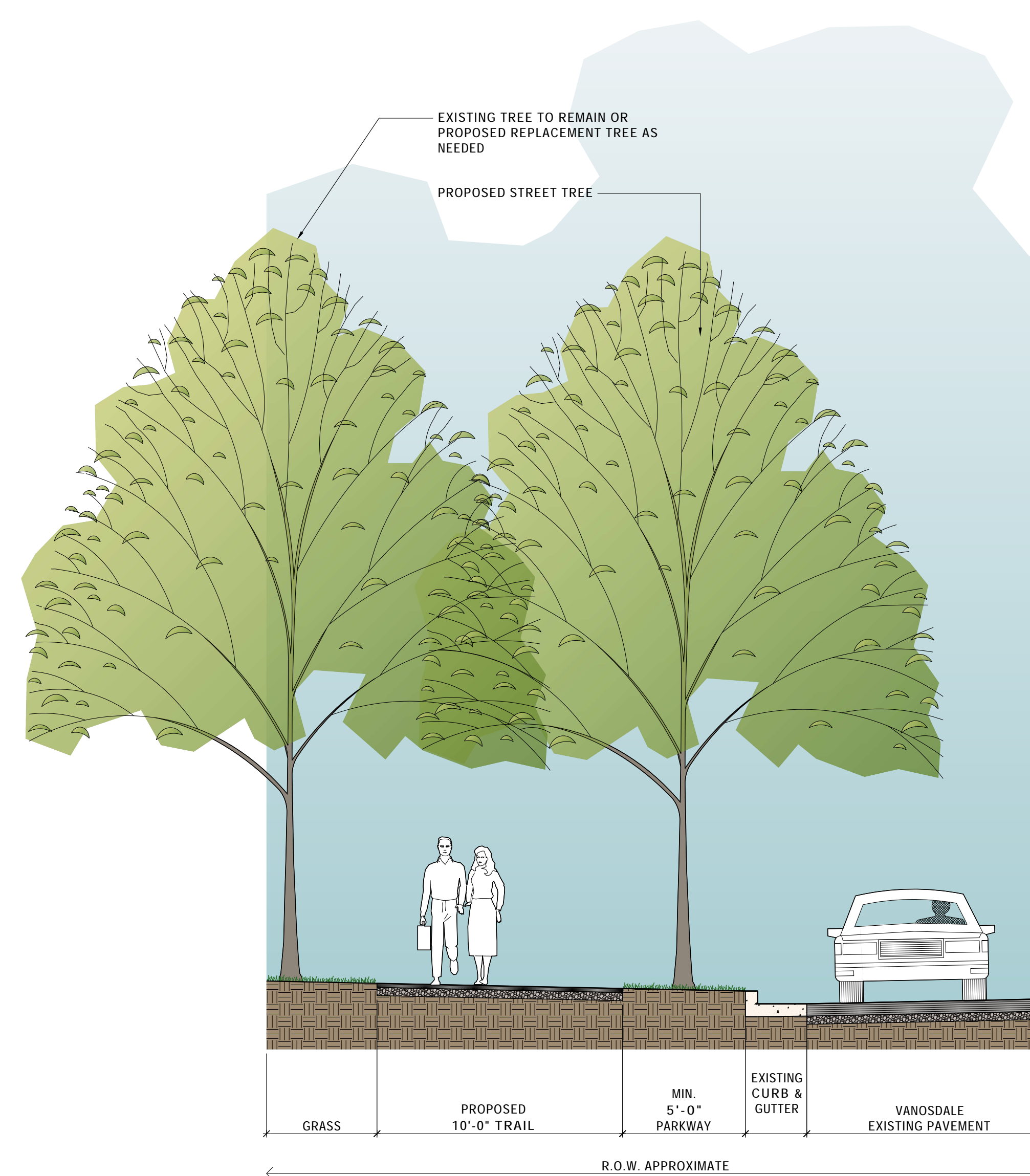
1 TYPICAL SIDE PATH WITH PARKWAY SECTION SCALE: 1/4"=1'-0" @ VANOSDALE ROAD
