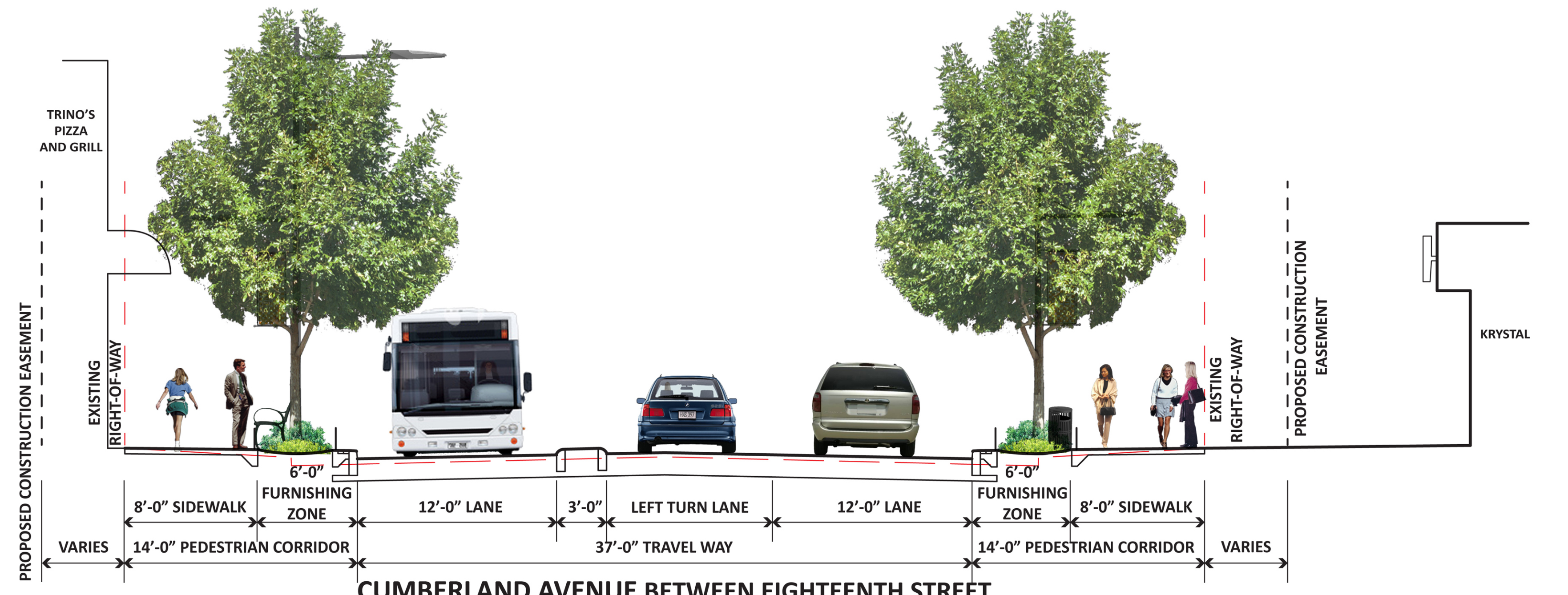
CUMBERLAND AVENUE BETWEEN EIGHTEENTH STREET AND SEVENTEENTH STREET (SECTION D-D)
