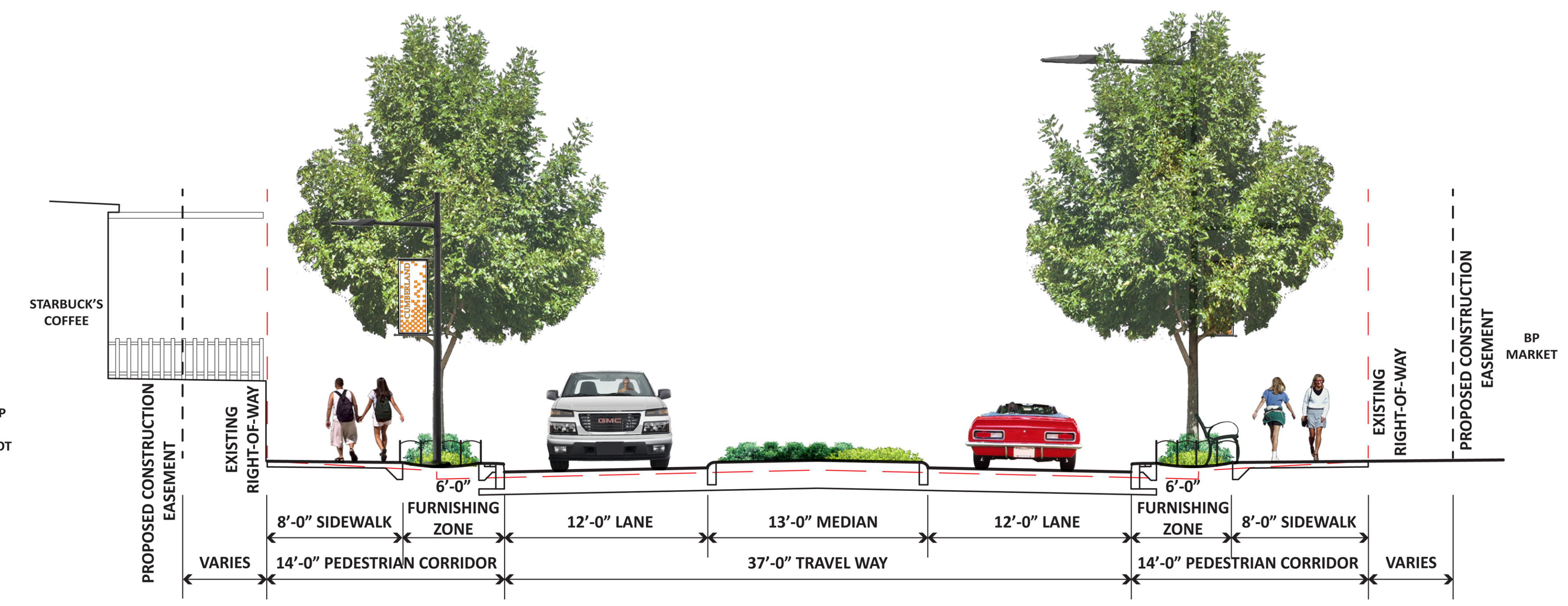
CUMBERLAND AVENUE BETWEEN TWENTY-FIRST STREET AND TWENTIETH STREET (SECTION B-B)
