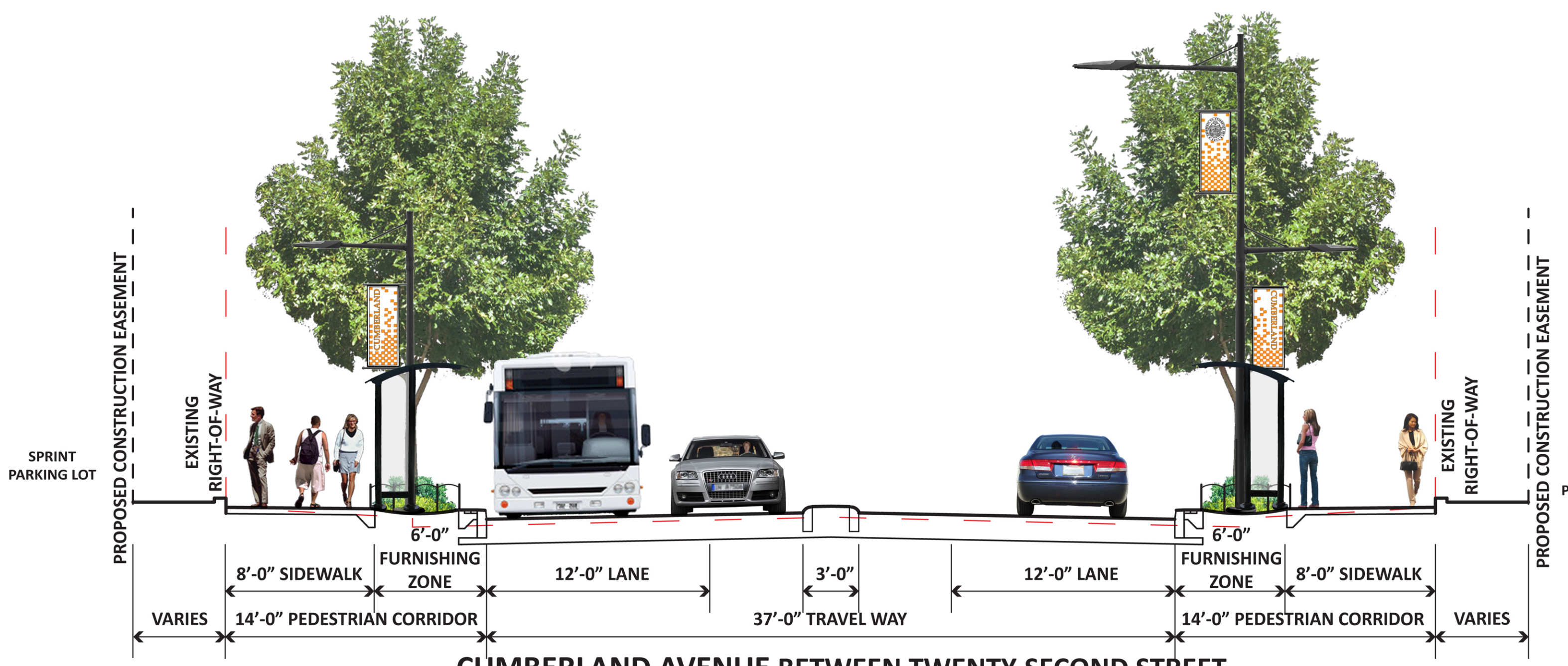
CUMBERLAND AVENUE BETWEEN TWENTY-SECOND STREET AND TWENTY-FIRST STREET (SECTION A-A)
