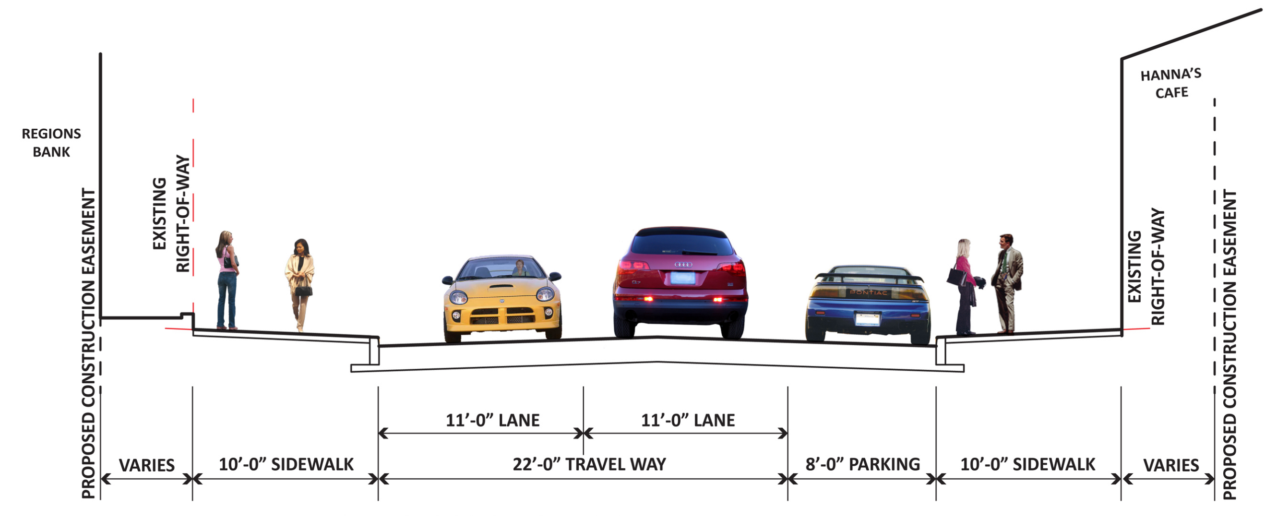
N NINETEENTH STREET BETWEEN WHITE AVENUE AND CUMBERLAND AVENUE (SECTION C-C)
