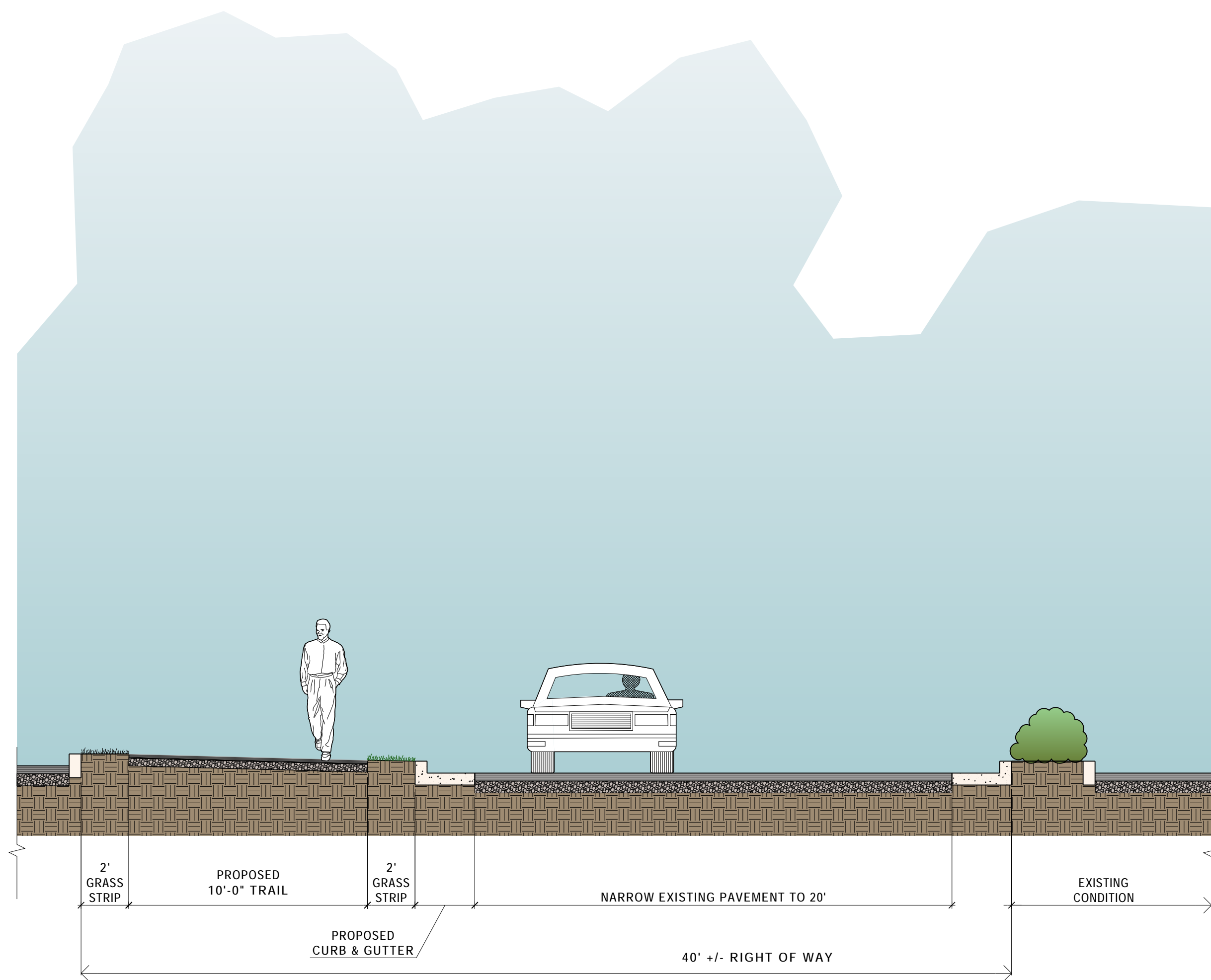
10 TRAIL ALONG GORE SCALE: 1/4"=1'-0"
