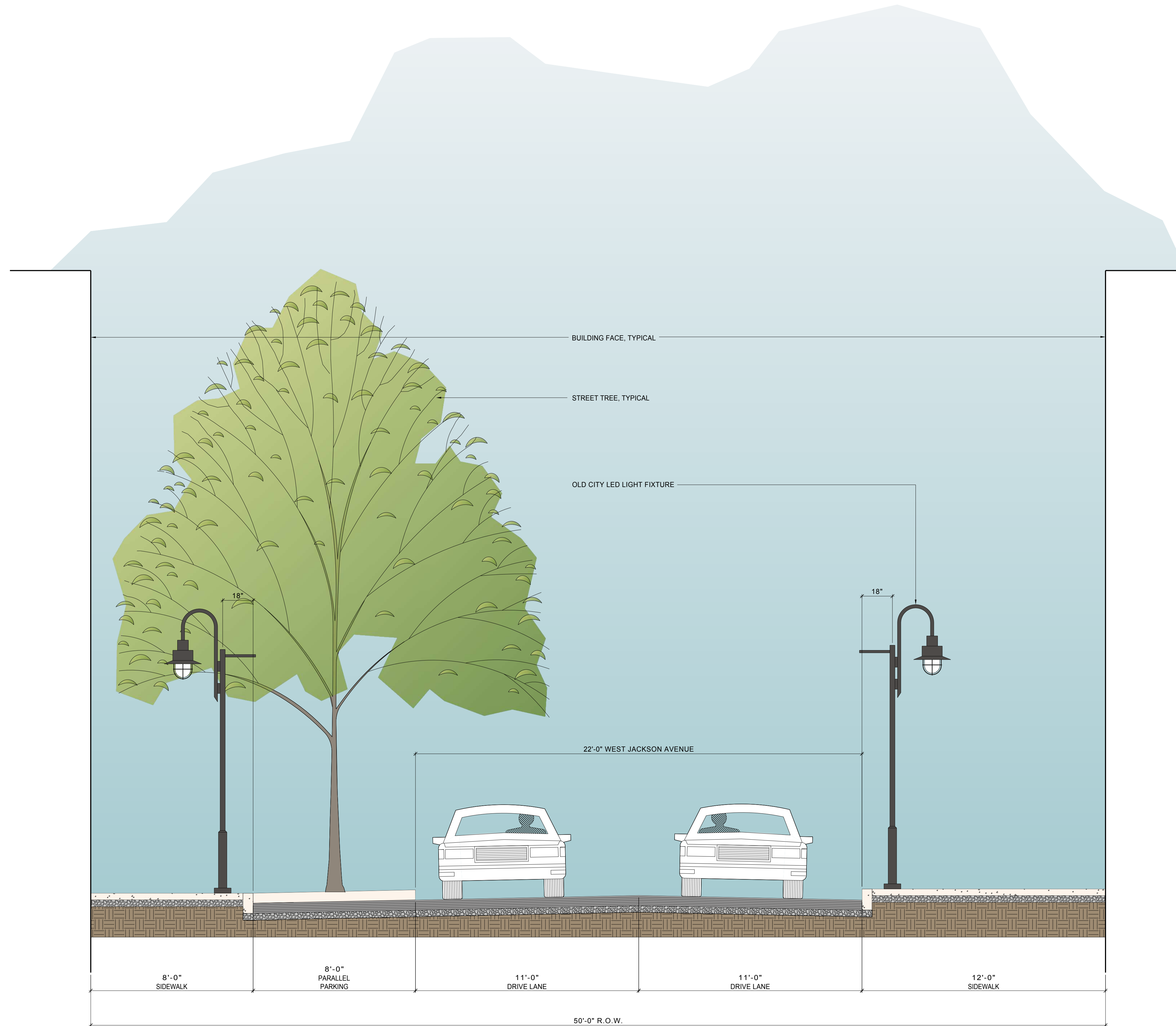
WEST JACKSON AVENUE STREETSCAPE SECTION SCALE: 3/8"=1'-0"
