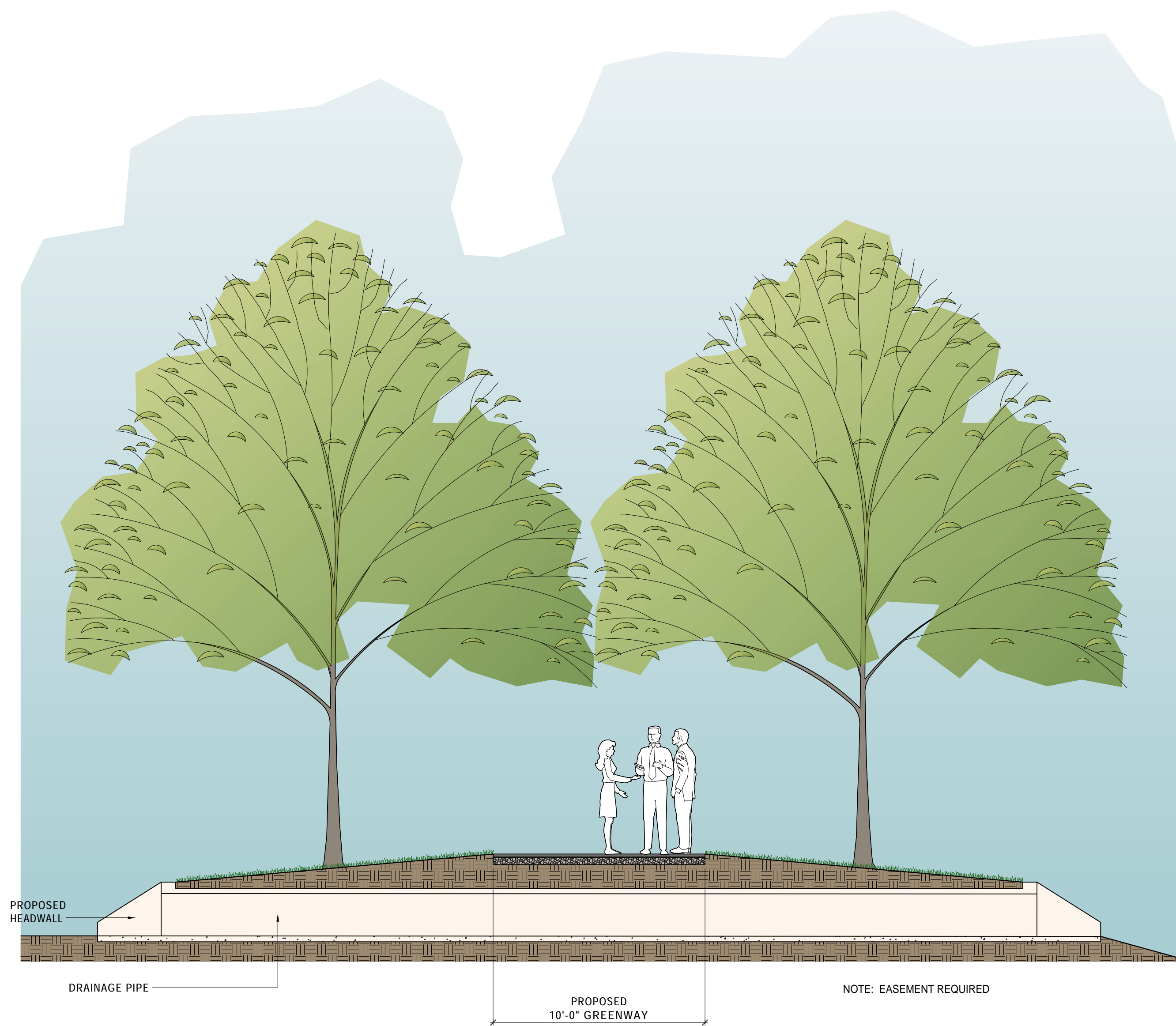
2 GREENWAY SECTION @ DRAINAGE CROSSING SCALE: 1/4"=1'-0"
