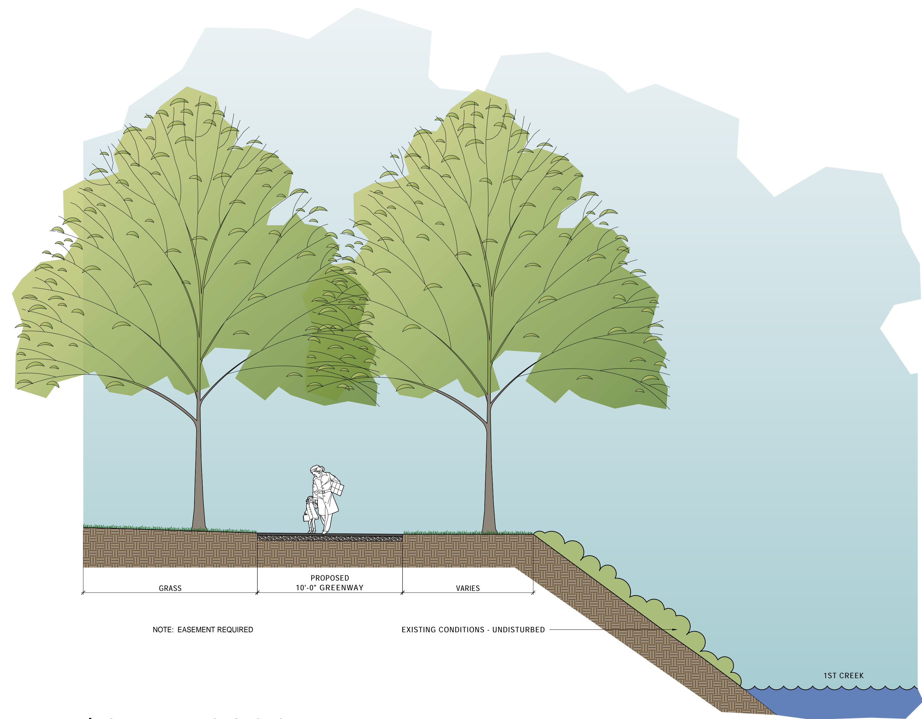
1 GREENWAY ALONG 1ST CREEK SCALE: 1/4"=1'-0"
